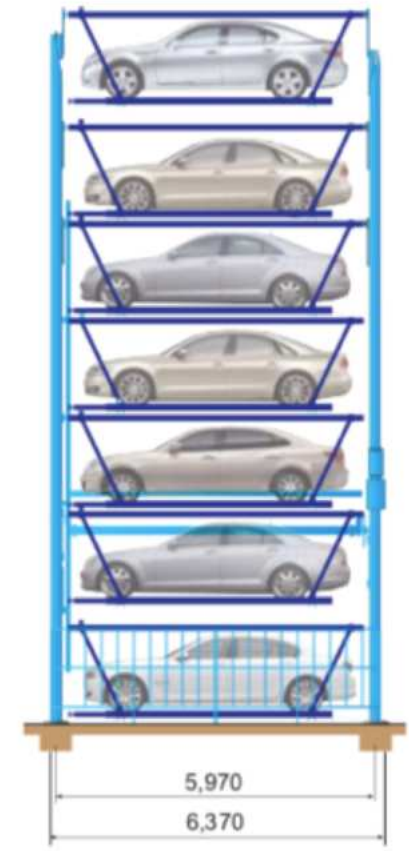
SIDE ELEVATION
